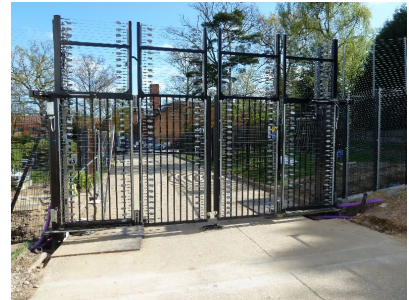
Example 2 Bi-Folding Speed Gate (Rack and Pinion)
